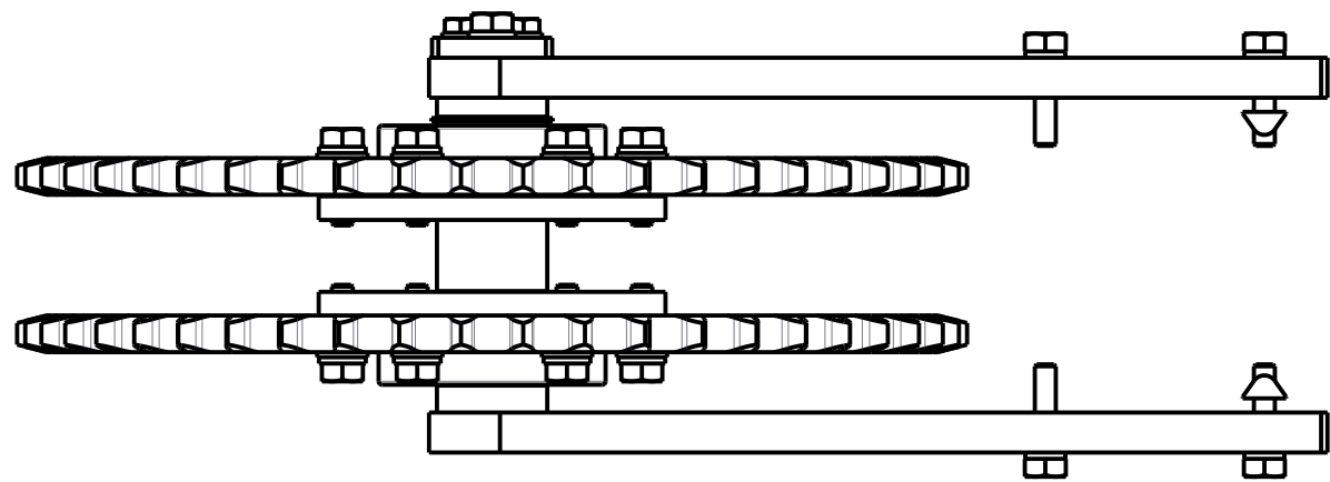
TOP ASSEMBLY VIEW SCALE 3/8
